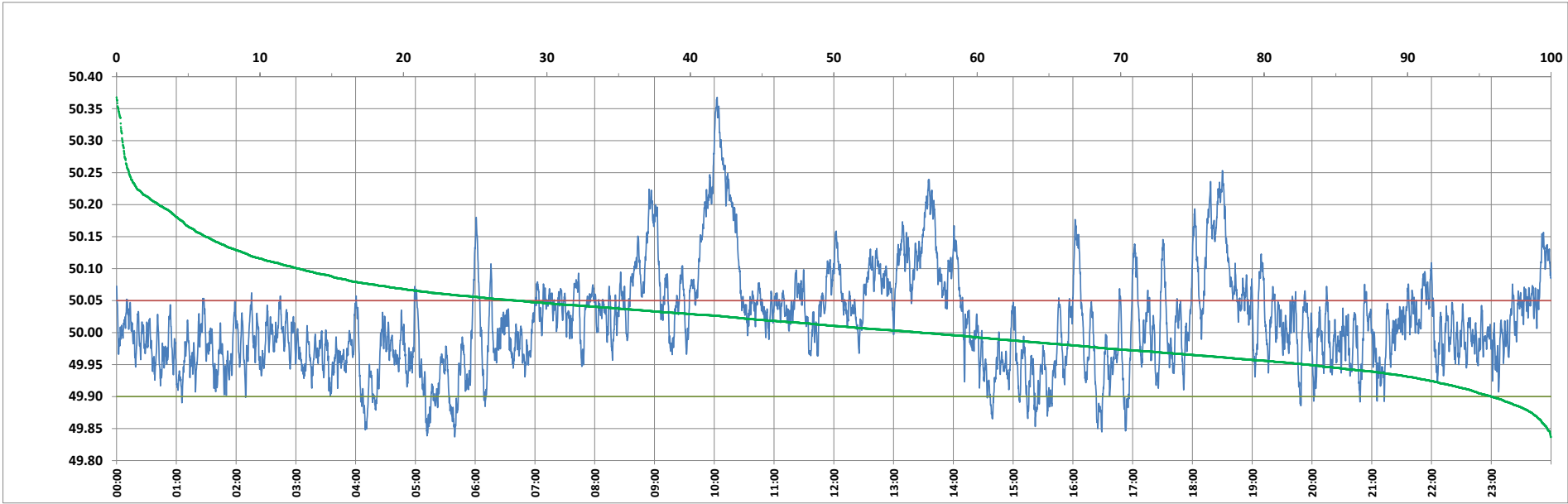
Frequency profile for 12-Nov-2023 (Sunday)
