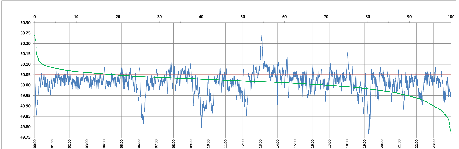
Frequency profile for 11-Aug-2023 (Friday)
