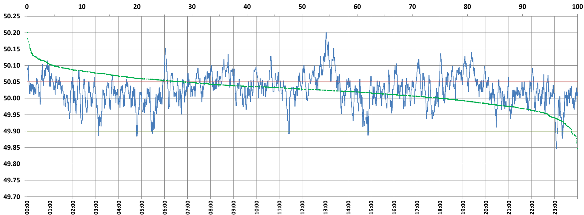
Frequency profile for 28-Sep-2021 (Tuesday)
