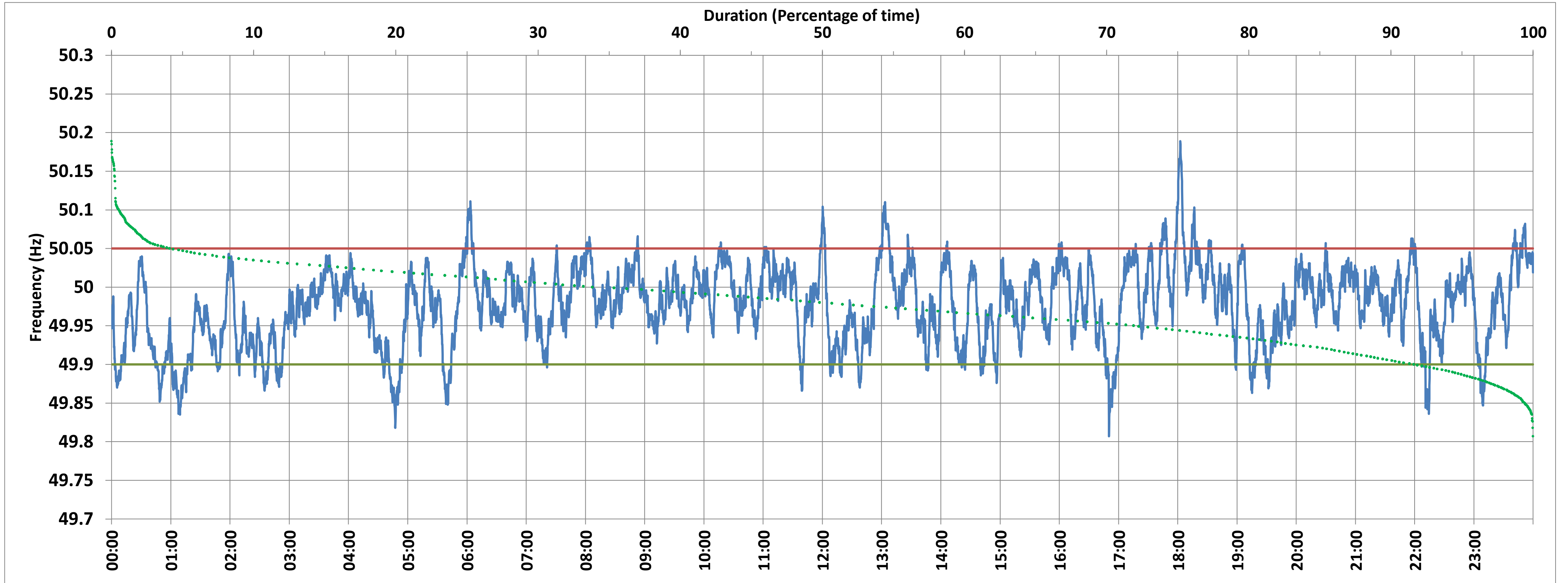
National Grid Frequency Profile for 6-May-2018
