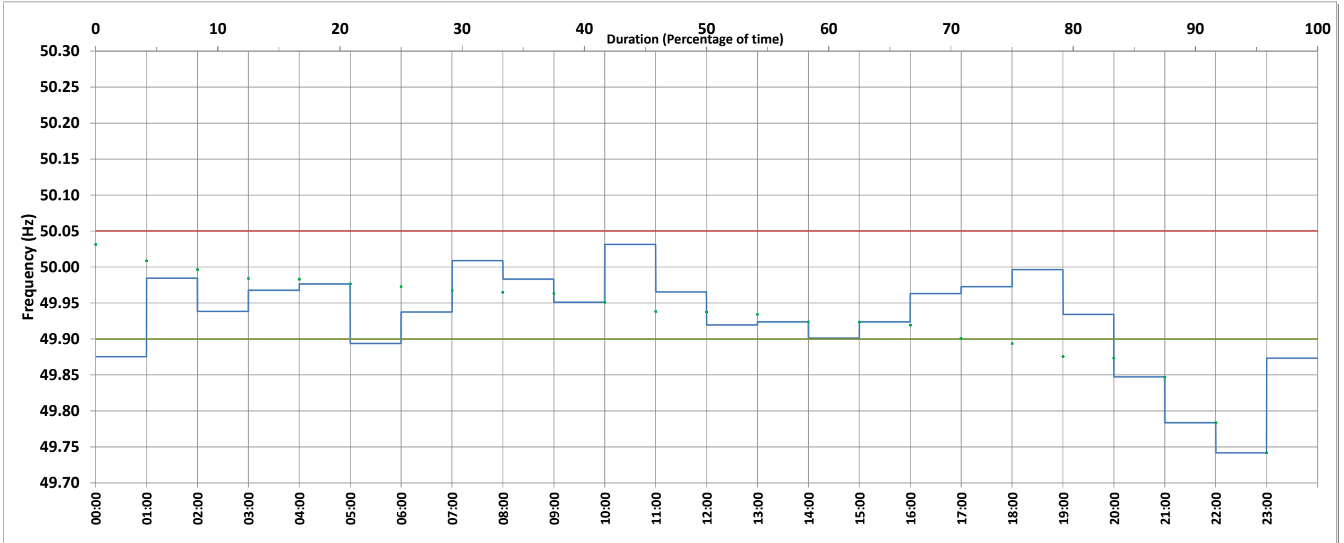
Hourly Average Frequency profile for 19-Jun-2018 (Tuesday)
