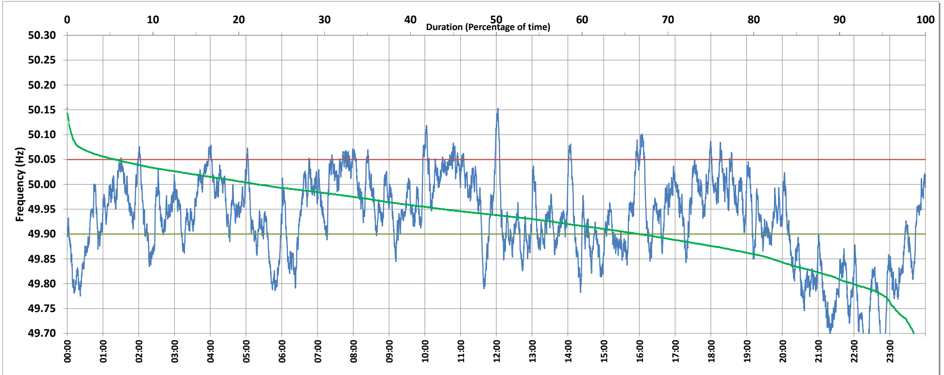
Frequency profile for 19-Jun-2018 (Tuesday)
