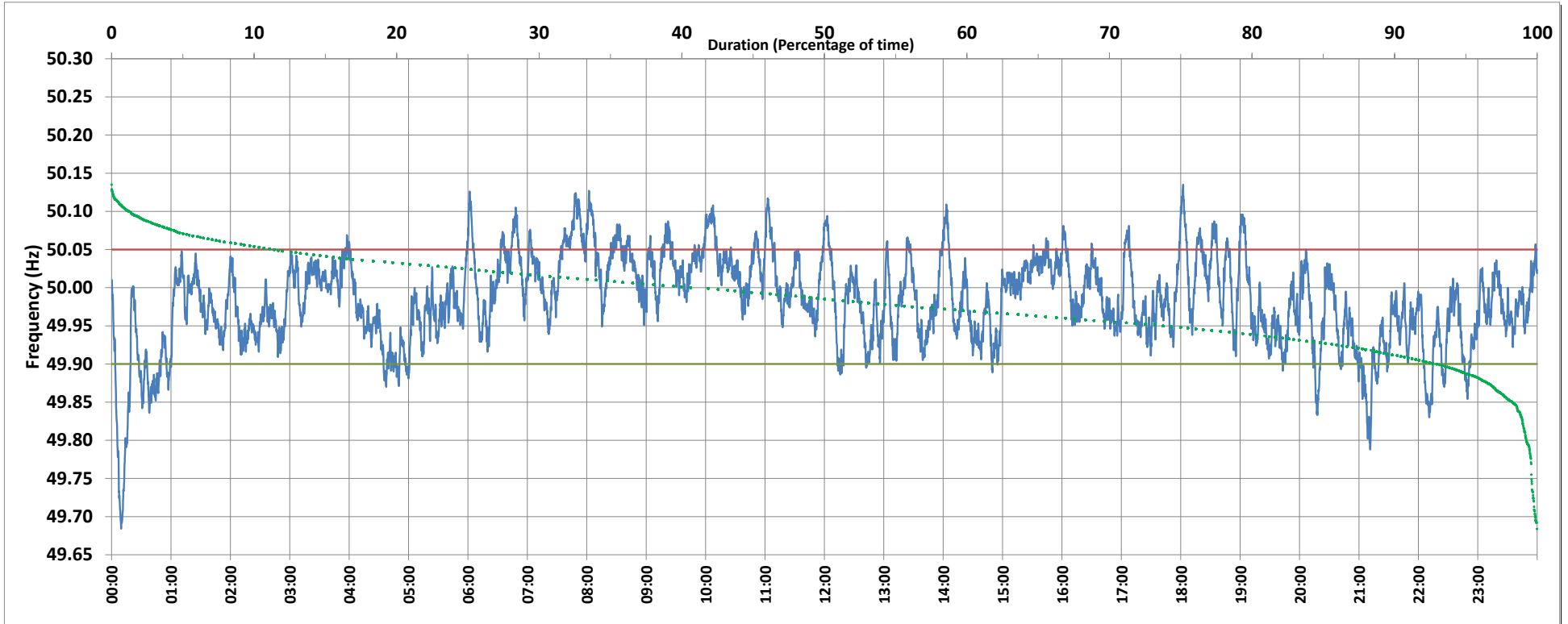
Frequency profile for 01-Jul-2018 (Sunday)
