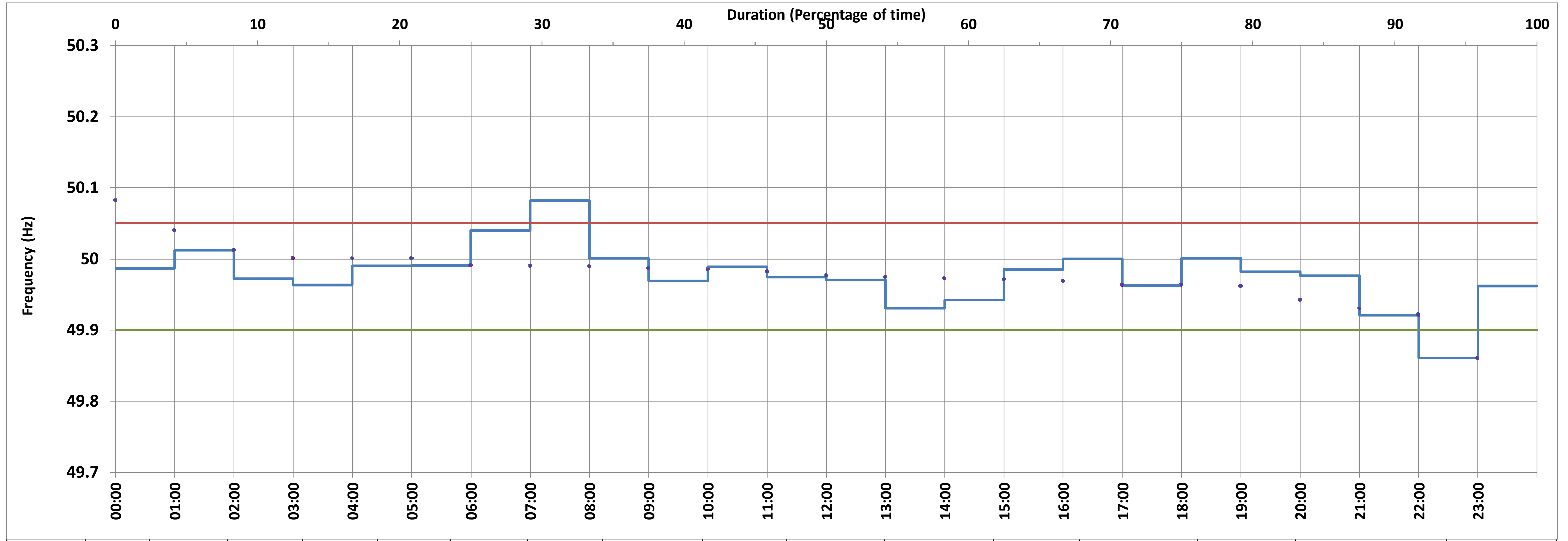
Hourly Average Frequency Profile for 9-Apr-2018
