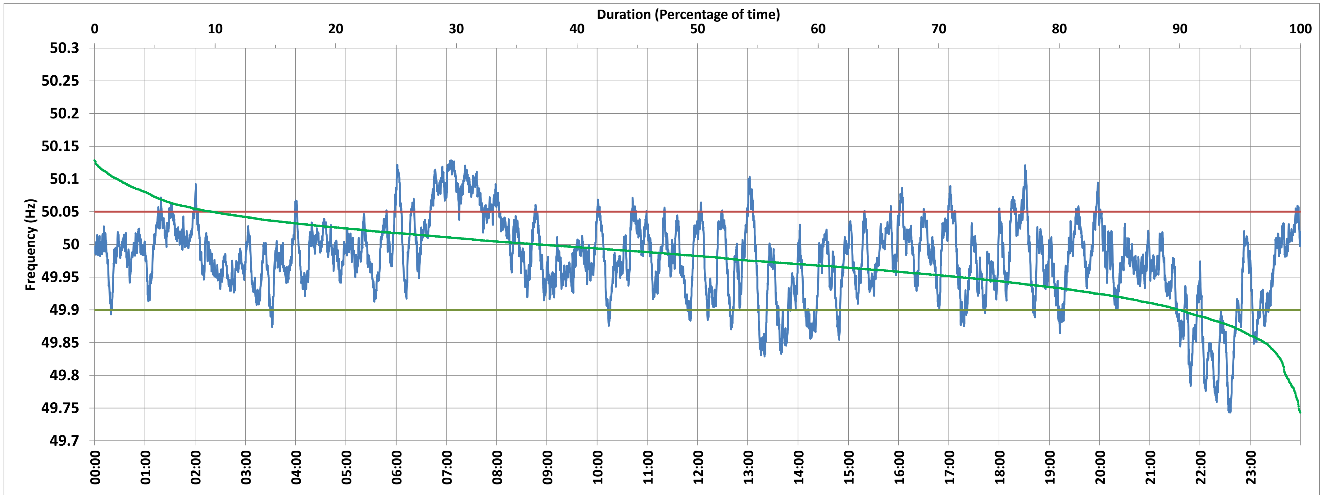
National Grid Frequency Profile for 9-Apr-2018
