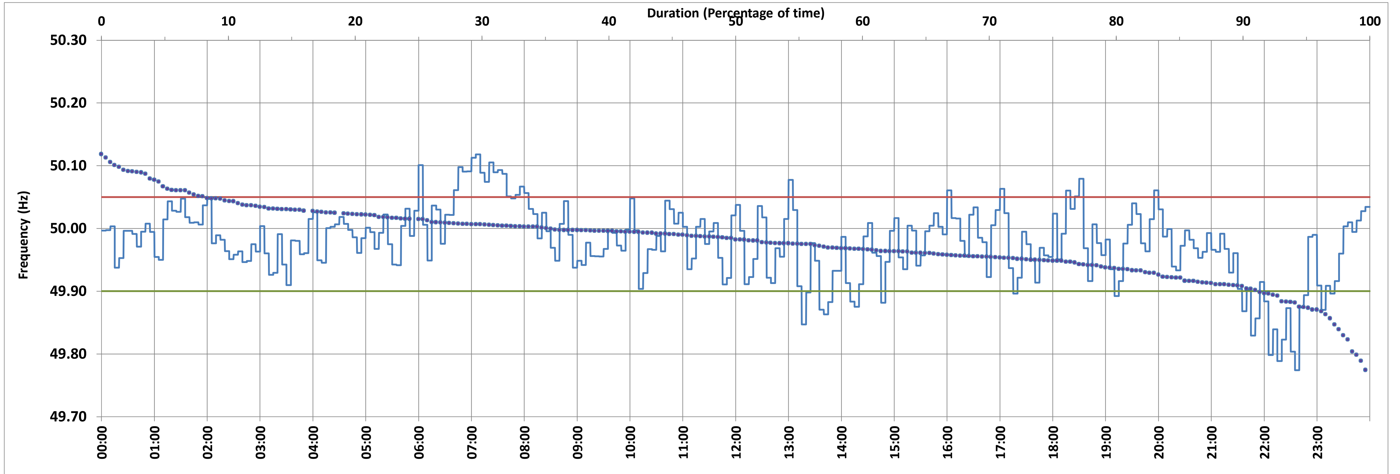
5 Min. Average Frequency Profile for 9-Apr-2018
