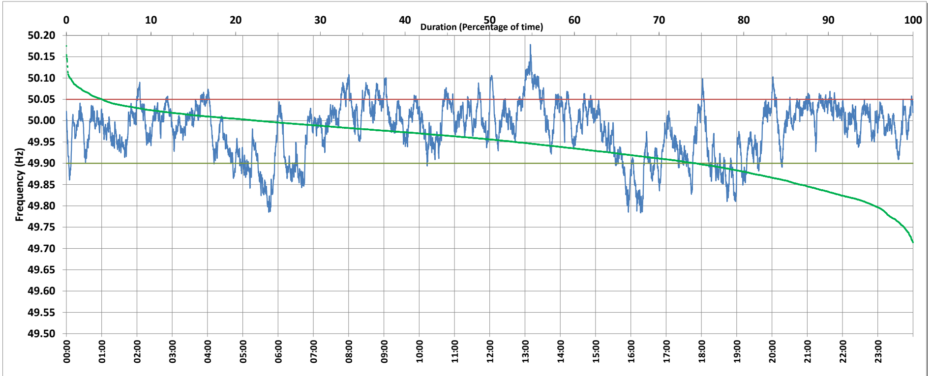
Frequency profile for 25-Sep-2018 (Tuesday)
