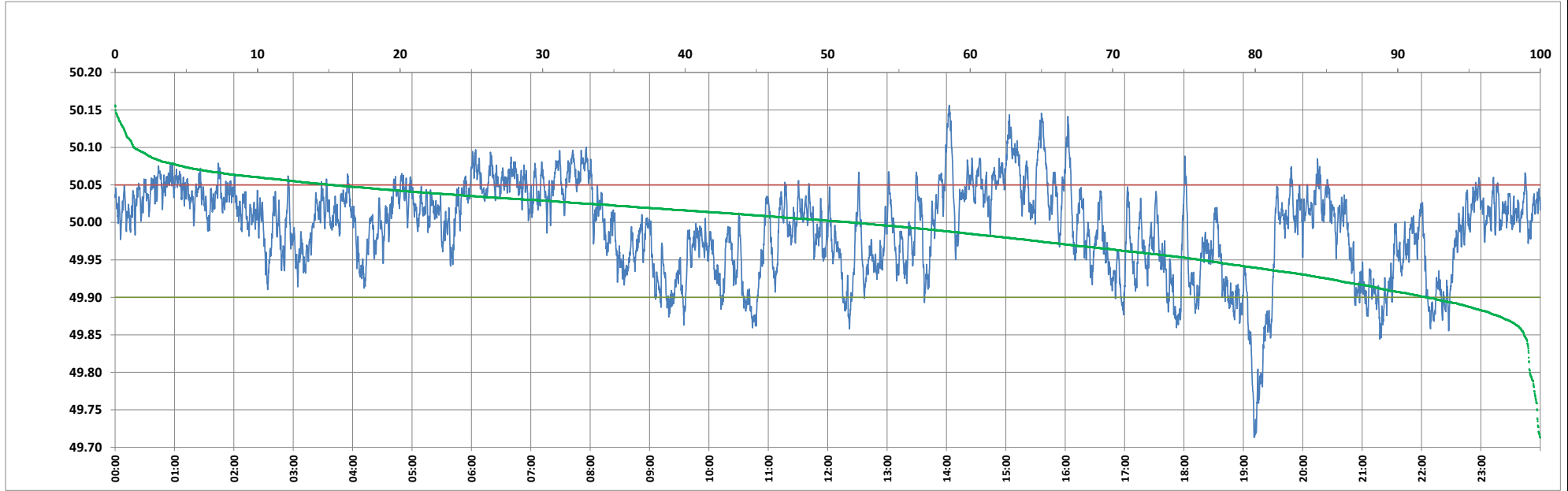
Frequency profile for 23-Jun-2024 (Sunday)
