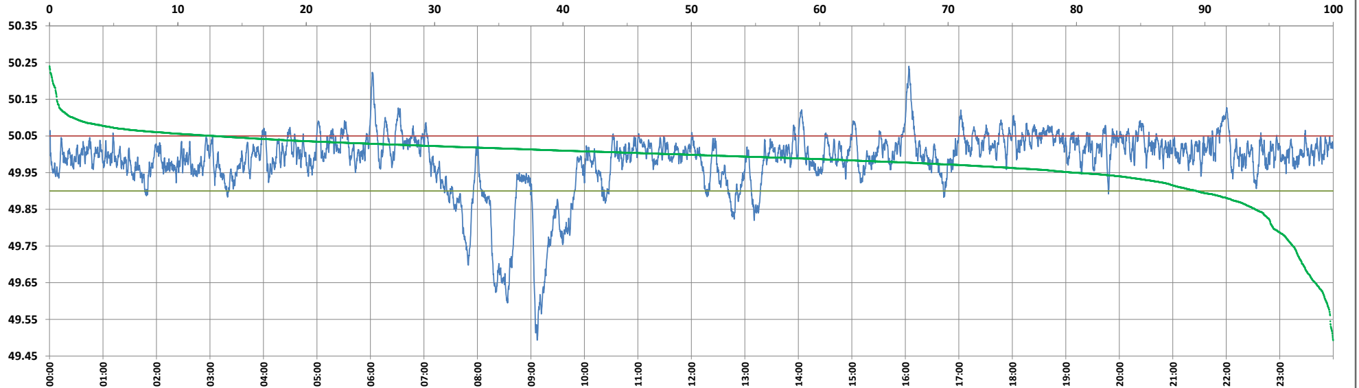
Frequency profile for 22-Dec-2024 (Sunday)
