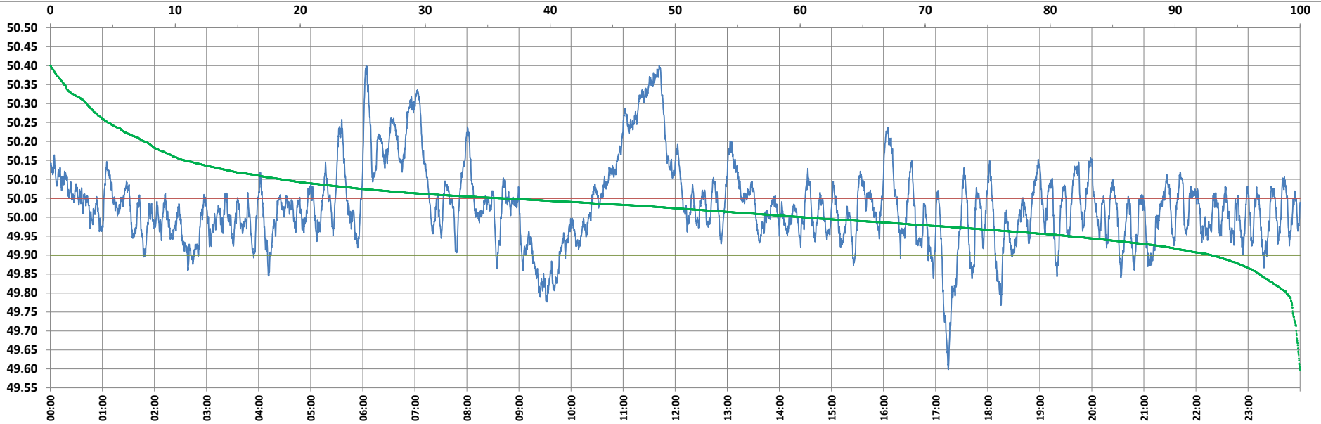
Frequency profile for 22-Dec-2022 (Thursday)
