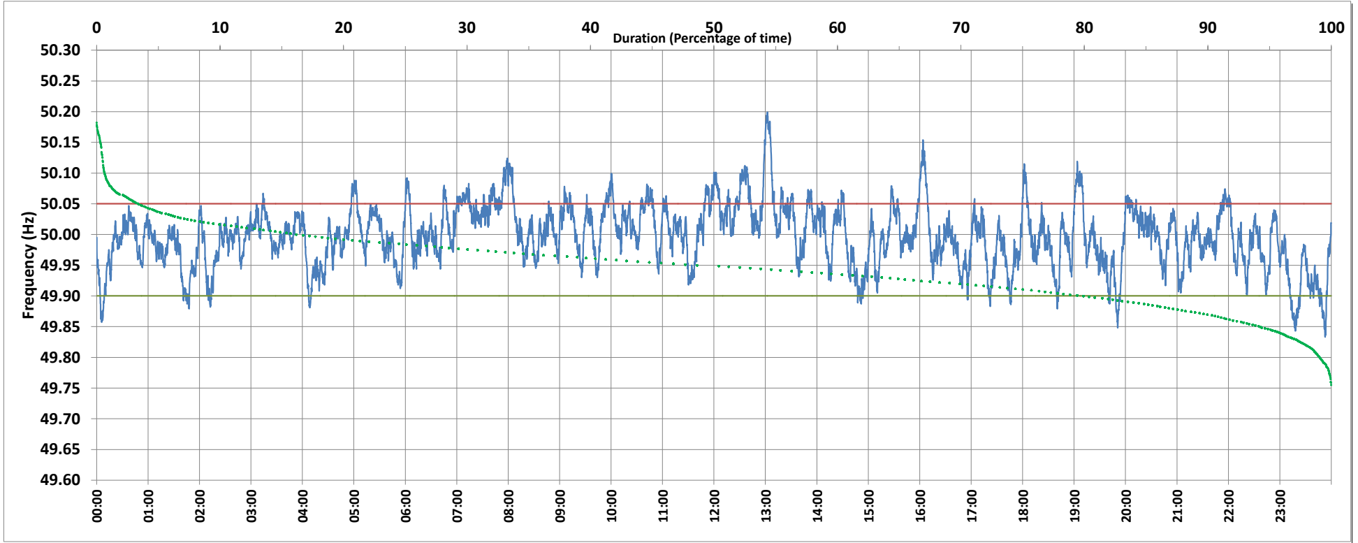
Frequency profile for 21-Jul-2018 (Saturday)
