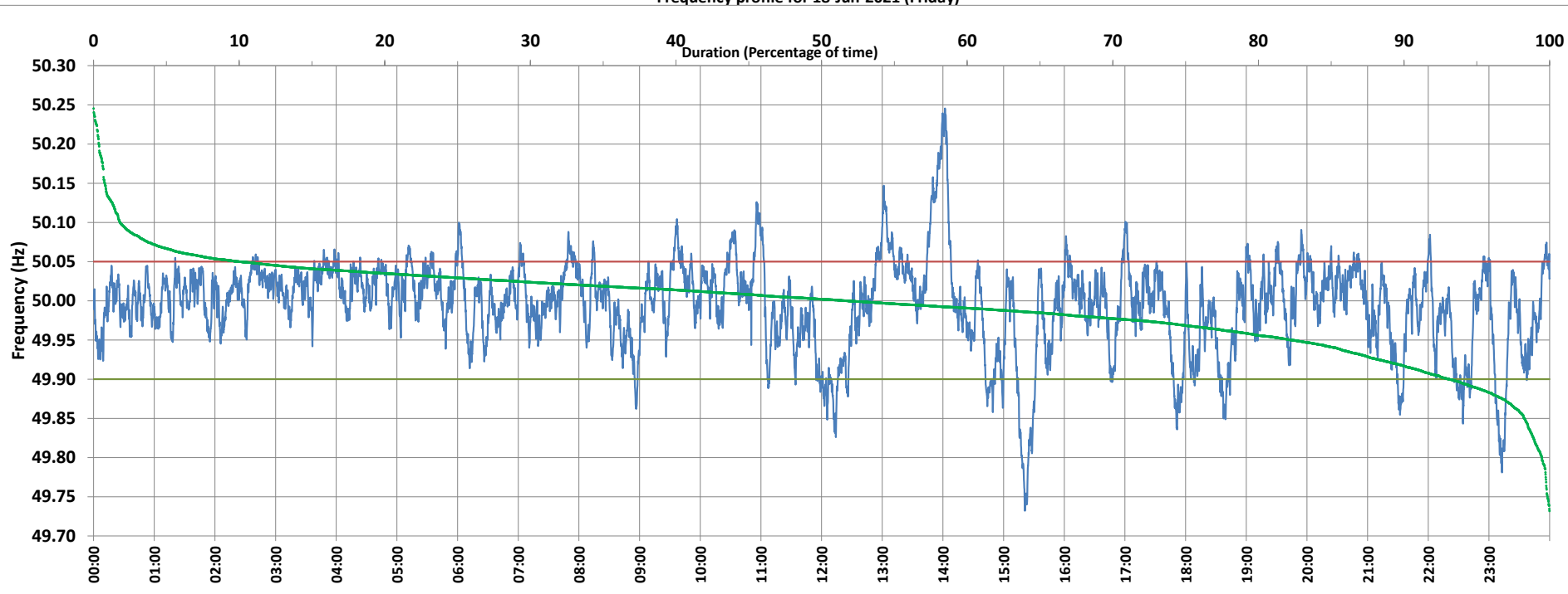
Frequency profile for 18-Jun-2021 (Friday)
