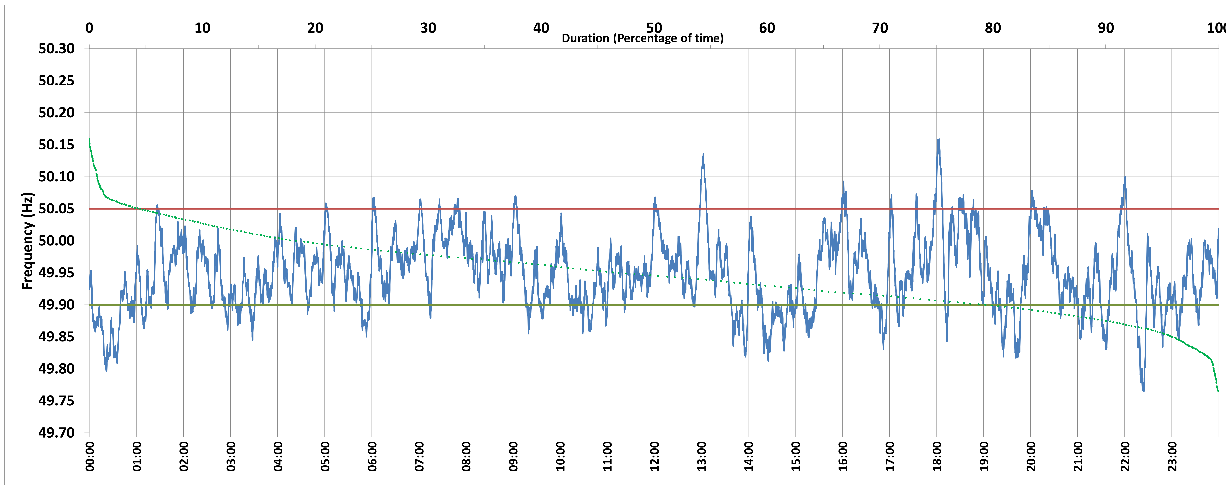
Frequency profile for 17-May-2018 (Thursday)
