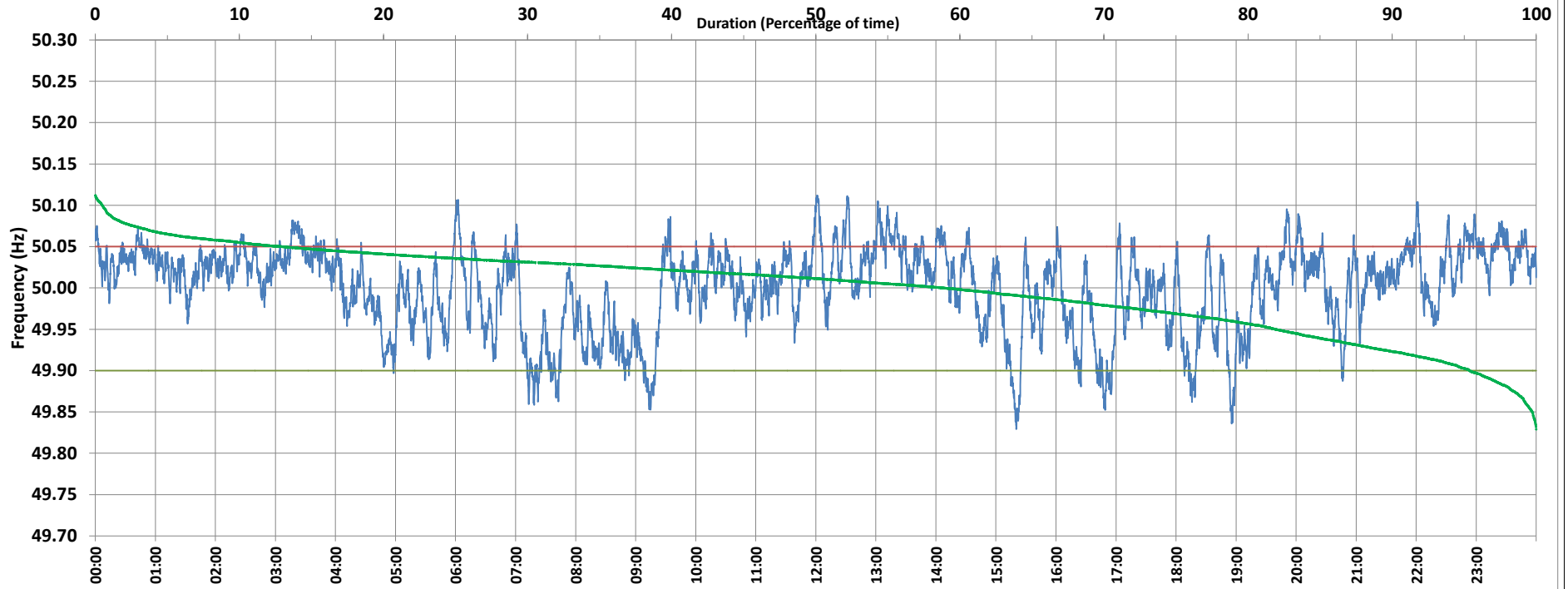
Frequency profile for 14-Sep-2020 (Monday)
