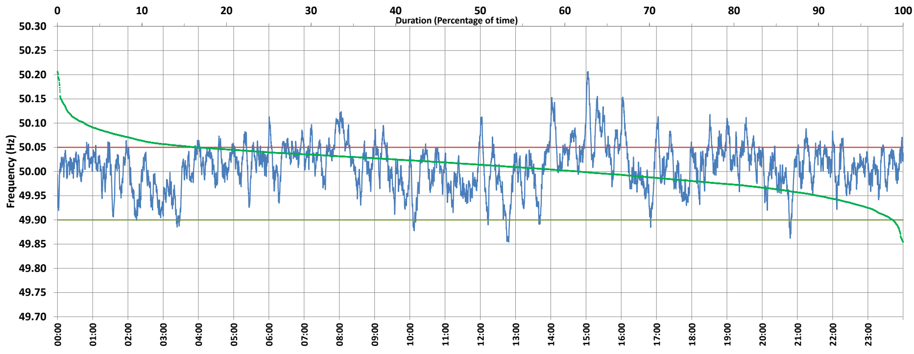
Frequency profile for 09-May-2021 (Sunday)
