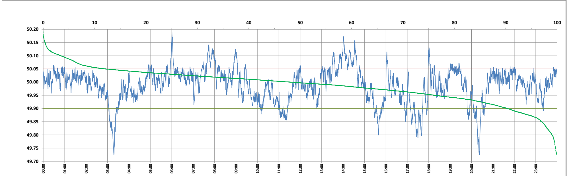
Frequency profile for 06-Oct-2024 (Sunday)
