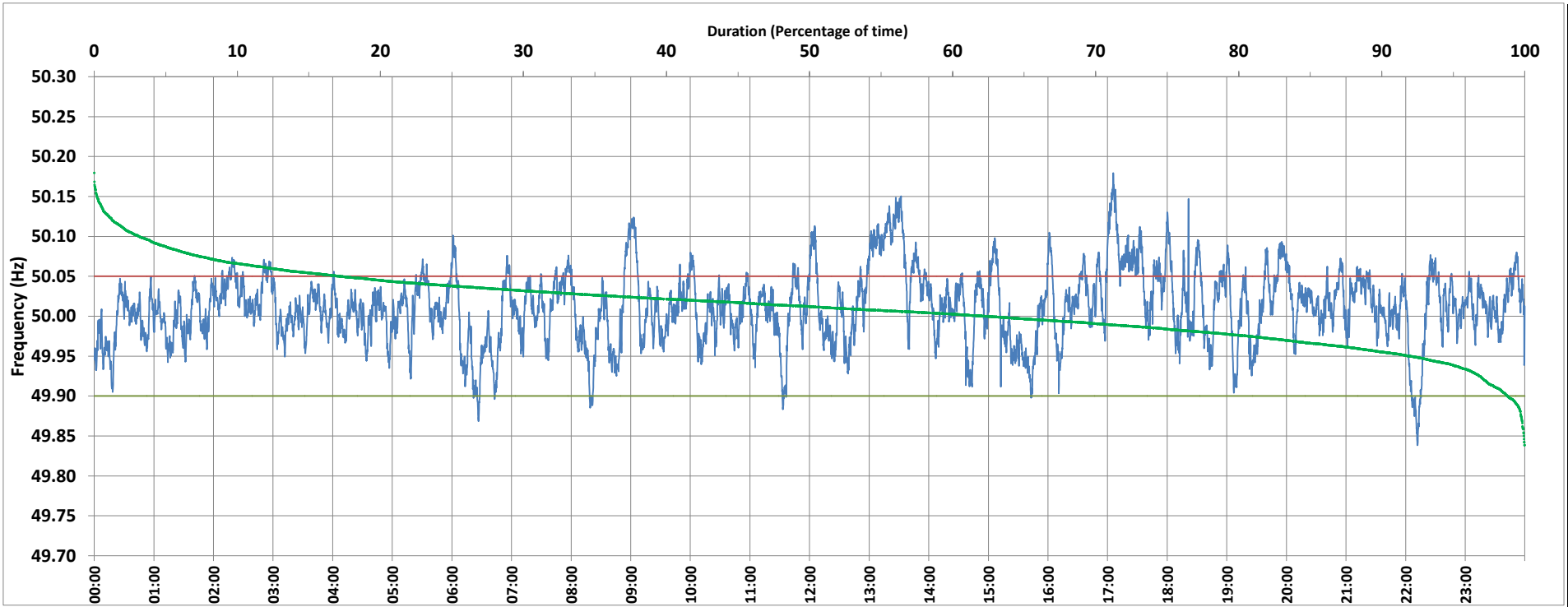
Frequency profile for 05-Sep-2020 (Saturday)
