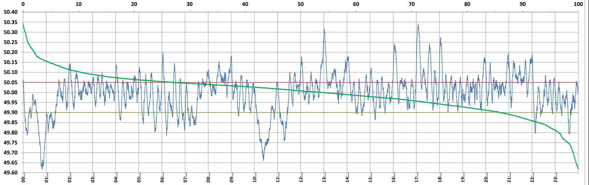
Frequency profile for 03-Feb-2023 (Friday)
